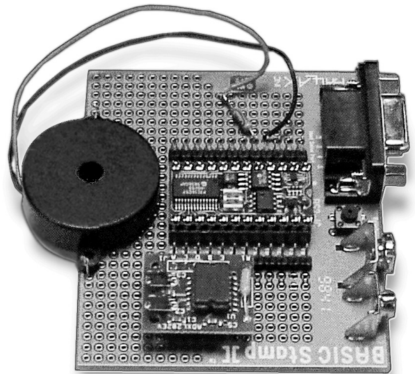
Figure 1. BASIC Stamp 2 Carrier Board and ADXL202EB
