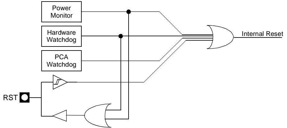
Figure 45. Reset schematic
