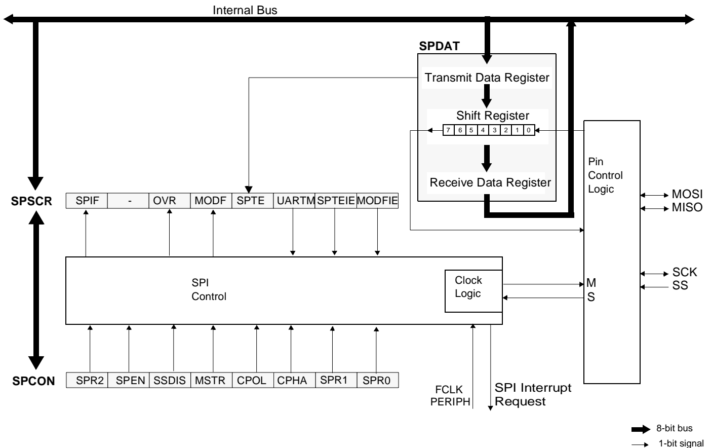
Figure 34. SPI Module Block Diagram
