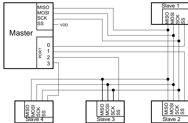
Figure 33. SPI Master/Slaves Interconnection
