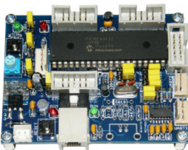
3. ET-BASE PIC40/46K22 (ICSP)
