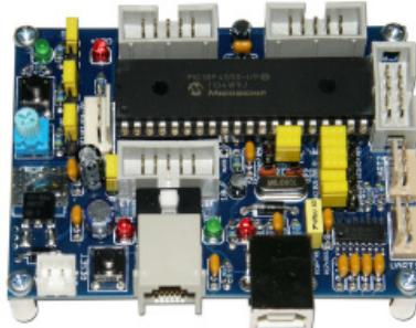
4. ET-BASE PIC40/46K80 (ICSP)
