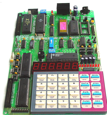
ET-BOARD V6.0
